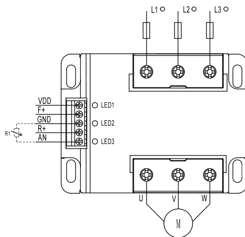
CMH...-24FT Series
