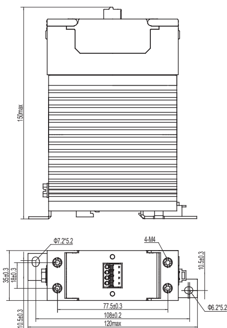
with KHS-P90 heat sink
