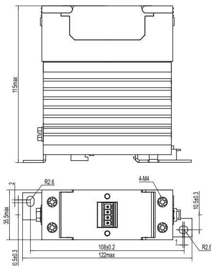
with KHS-H90 heat sink
